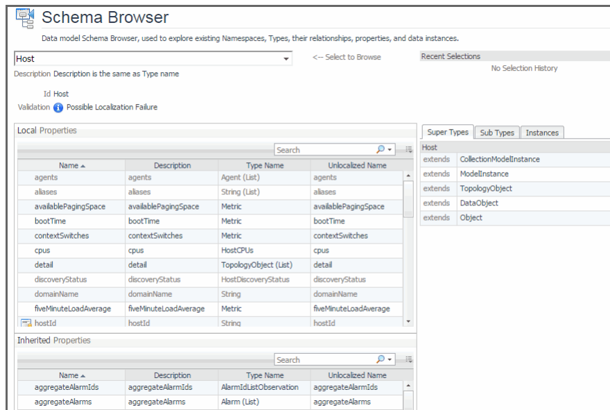
Figure 1. Schema Browser
