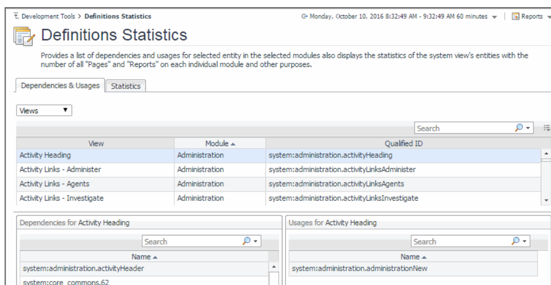
Figure 1. Definitions Statistics
