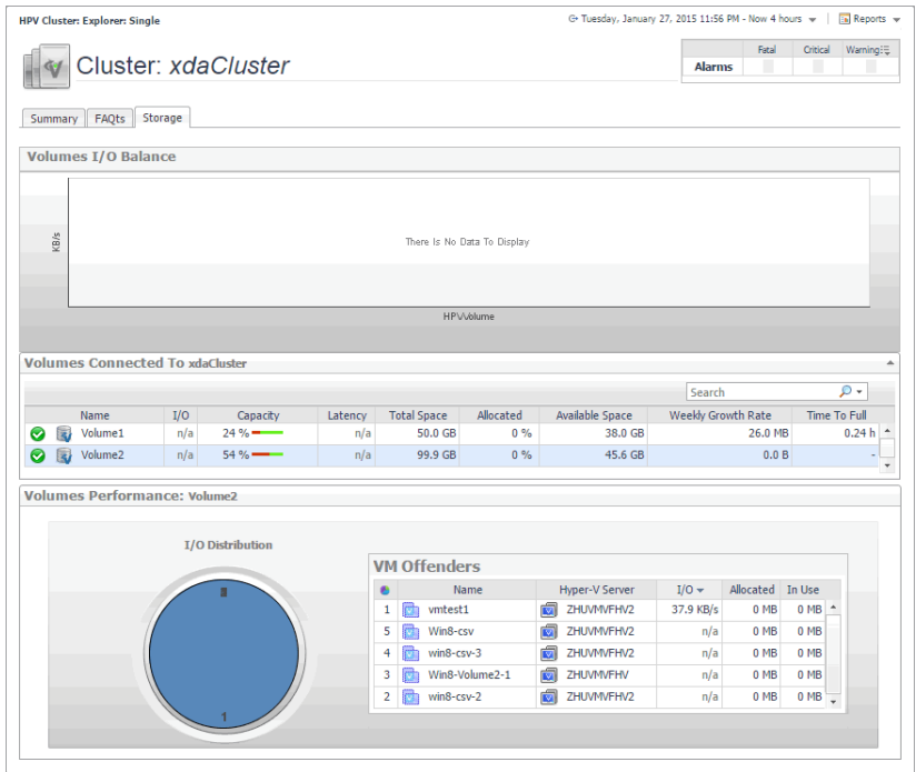
Figure 85. Storage tab (clusters)
