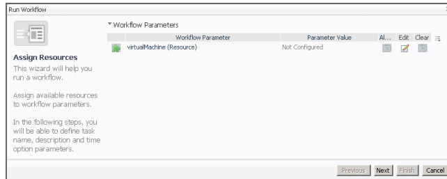
Figure 116. Run Workflow dialog box
