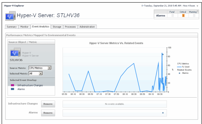
Figure 79. Event Analytics tab
