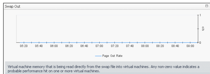
Figure 49. Swap Out dialog box
