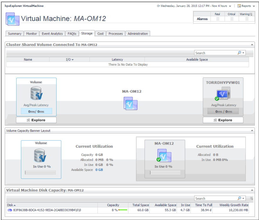
Figure 87. Storage tab (virtual machines)
