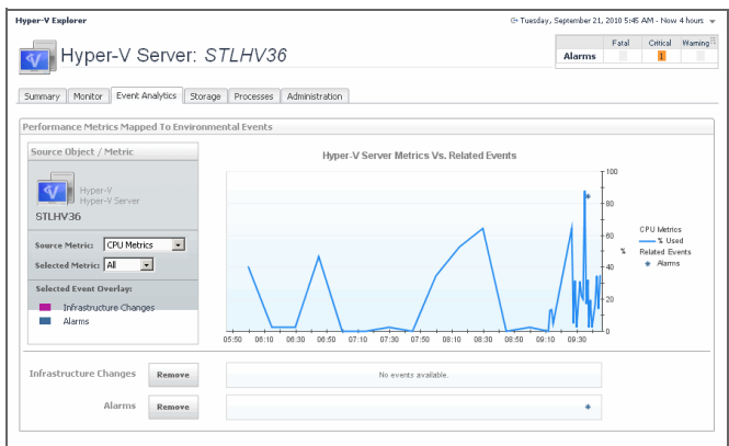
Figure 80. Event Analytics tab
