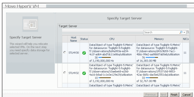
Figure 105. Move HyperV VM dialog box
