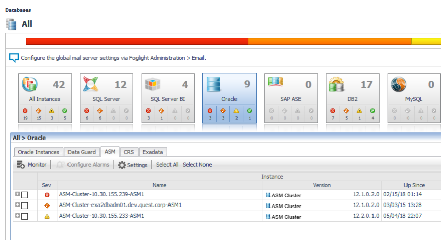
Figure 3. ASM tab
