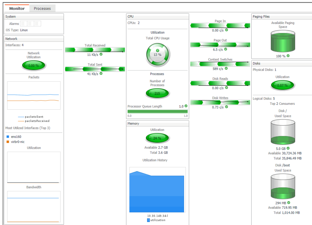
Figure 5. Exploring hosts
