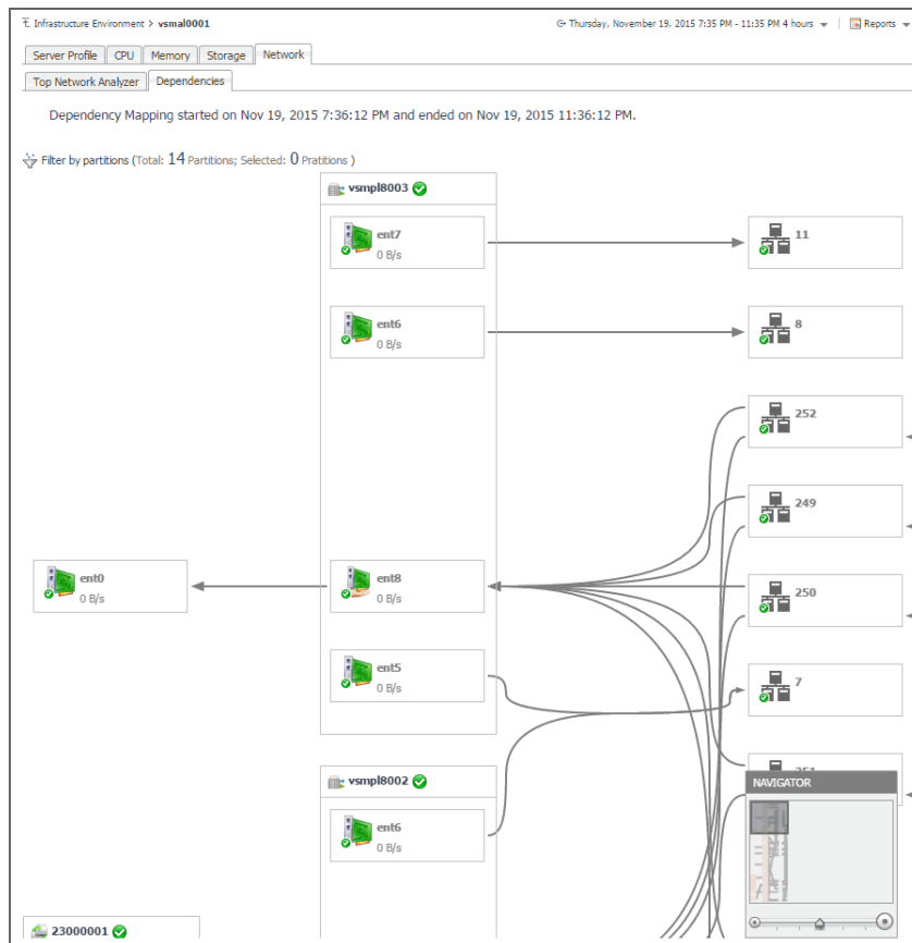
Figure 37. Dependency tab
