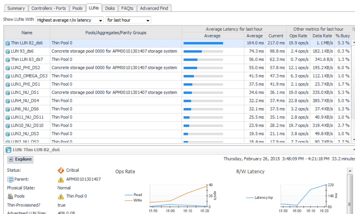
Figure 1. Performance Monitoring
