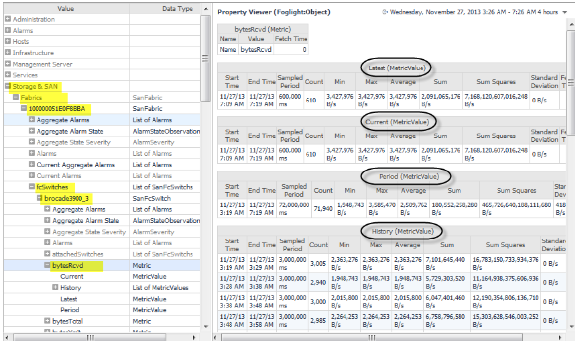
Figure 10. Property Viewer
