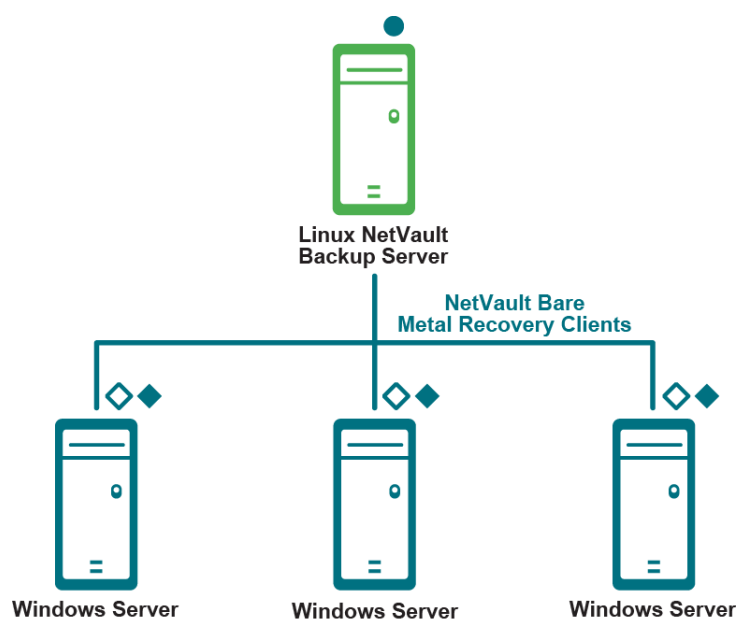
Figure 4. NetVault Bare Metal Recovery Client for Windows with Linux-based server
