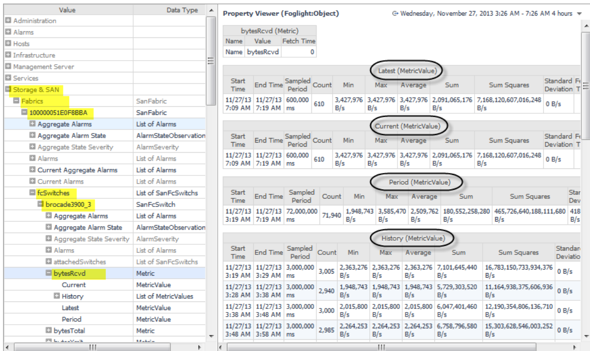
Figure 20. Property Viewer
