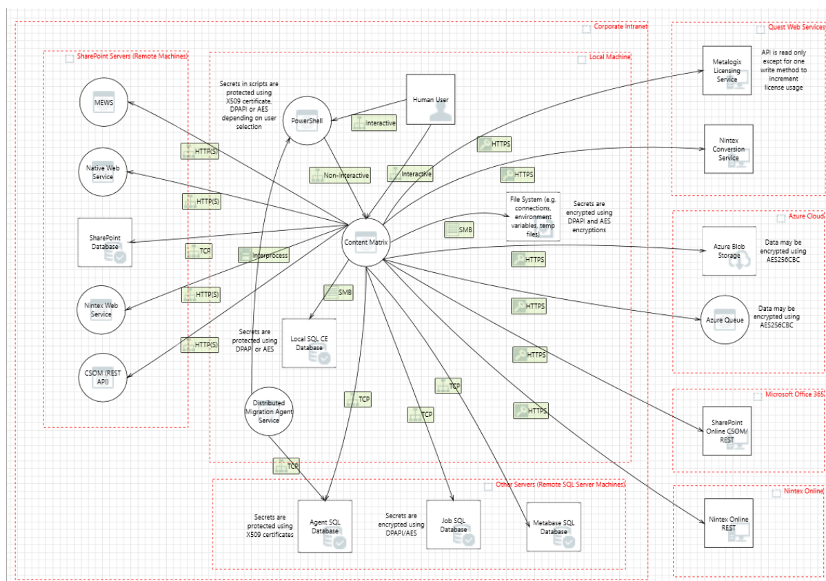
Figure 1: High-Level Architecture
