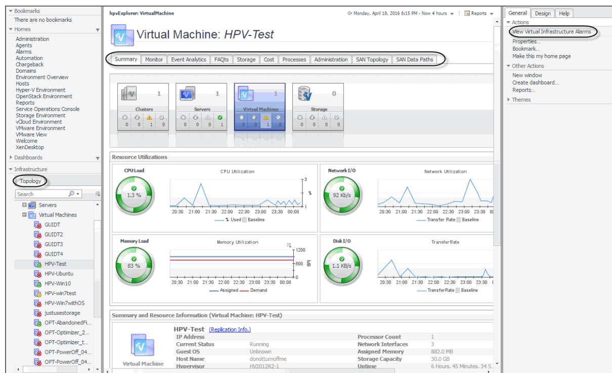
Figure 12. Hyper-V Explorer
