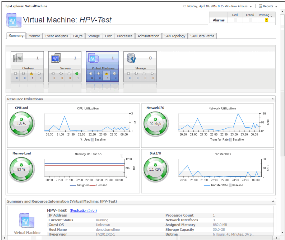
Figure 19. Summary tab
