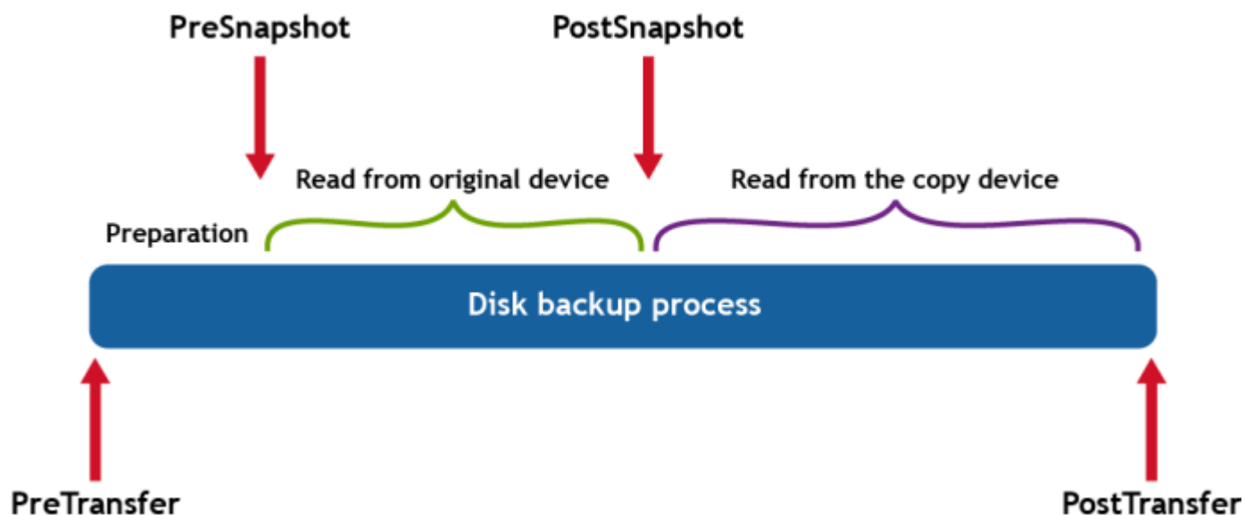
Figure 3. When pre and post scripts execute
