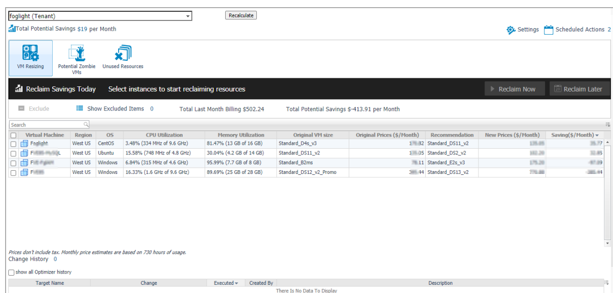
Figure 28. Optimizer tab
