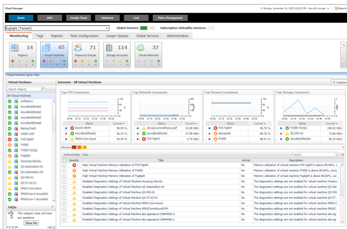
Figure 4. Monitoring dashboard
