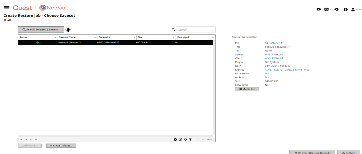
Figure 19. Create Restore Job — Choose Saveset page
