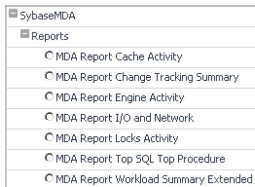
Figure 49. Reports
