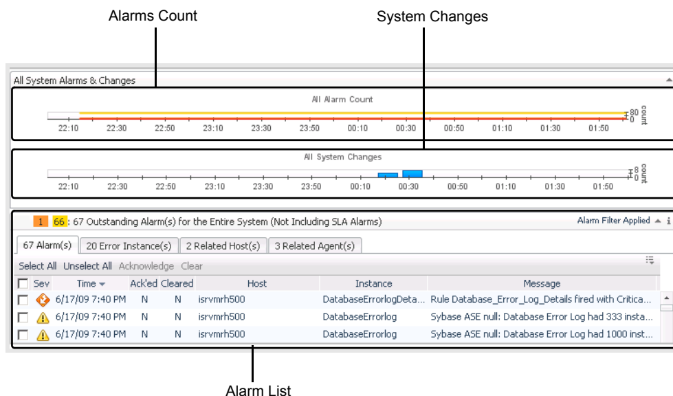
Figure 2. Alarms View
