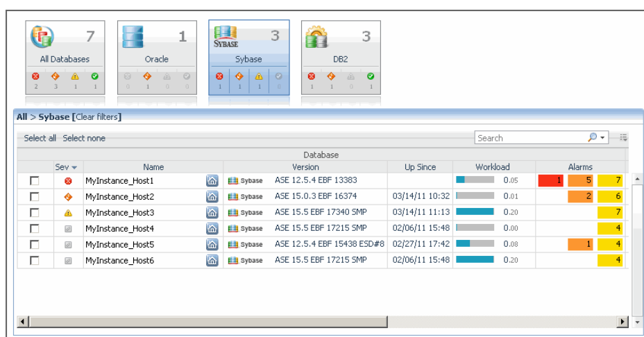
Figure 41. Database Instances
