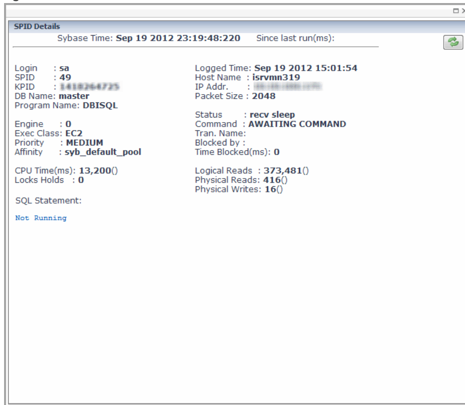
Figure 18. SPID Details
