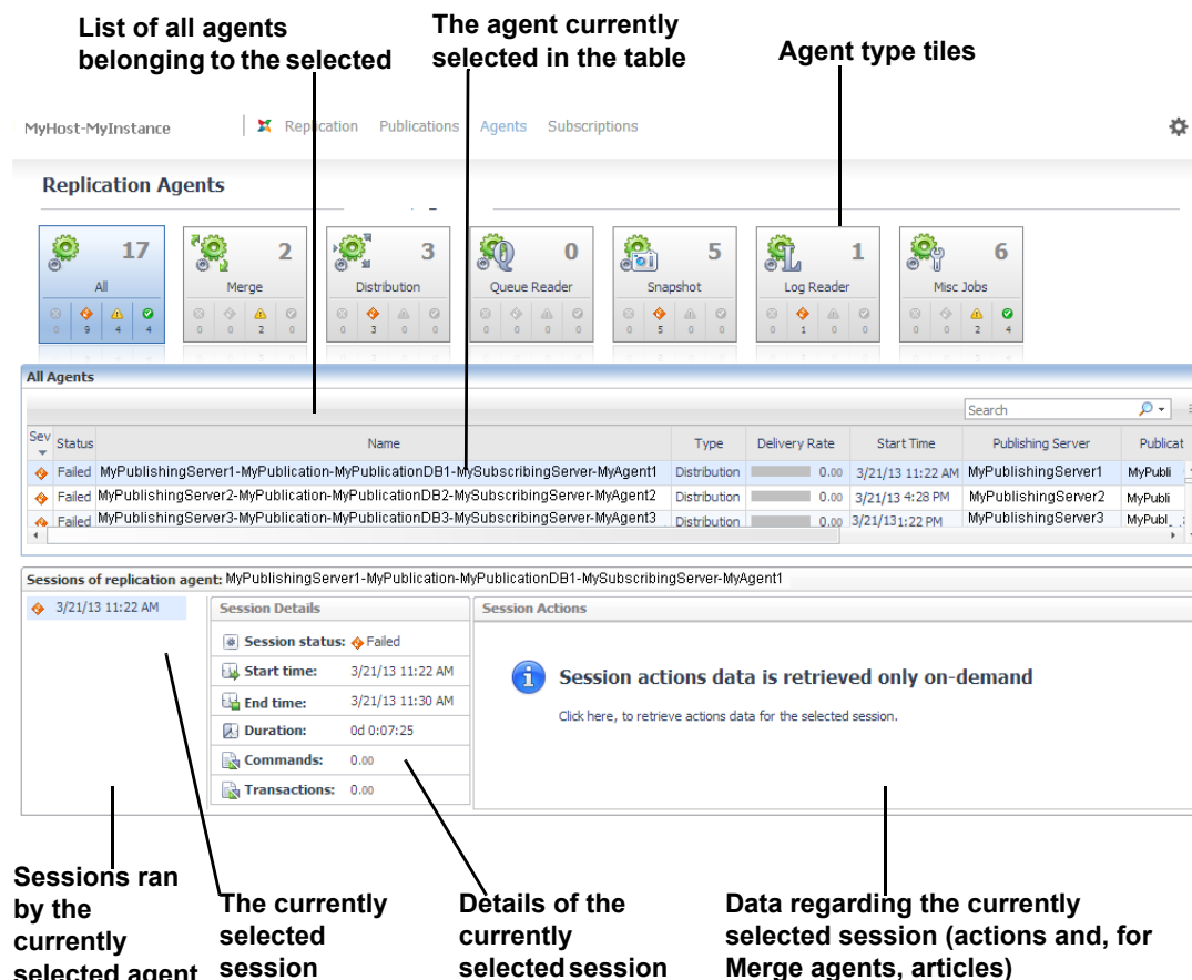
Figure 6. The Replication Agents drilldown.
