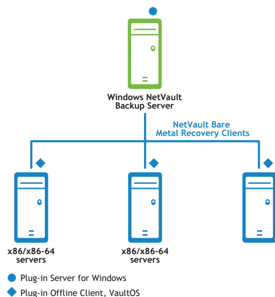
Figure 1. NetVault Bare Metal Recovery for offline only x86/x86-64 clients with Windows-based server
