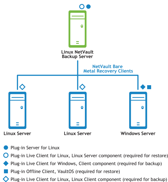
Figure 7. NetVault Bare Metal Recovery Client for Windows and Client for Linux with Linux-based server
